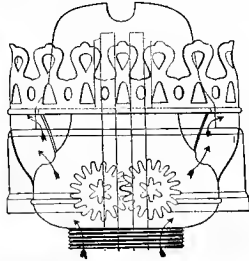
Figs. 3363-3364. Sectional Views. IMPROVED DUAL BURNERS, WITH SKIRT.
